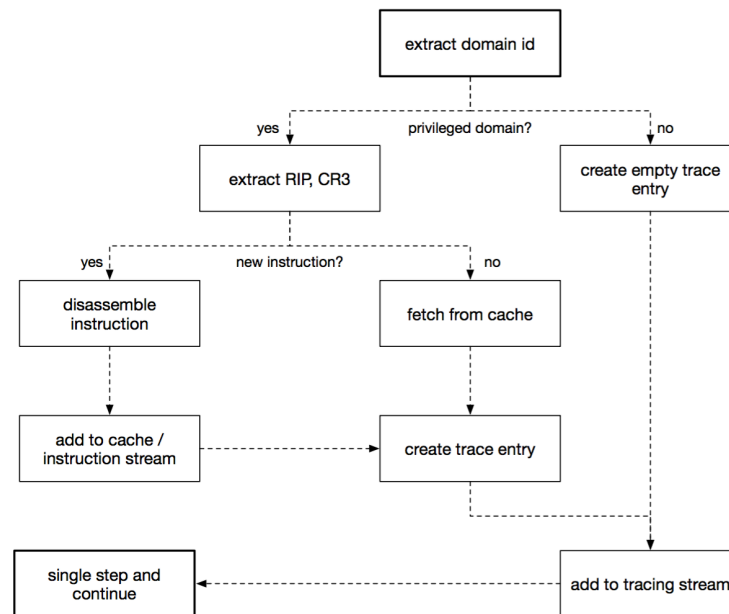
Figure 5-1. Decision tree for the callback handler function.
