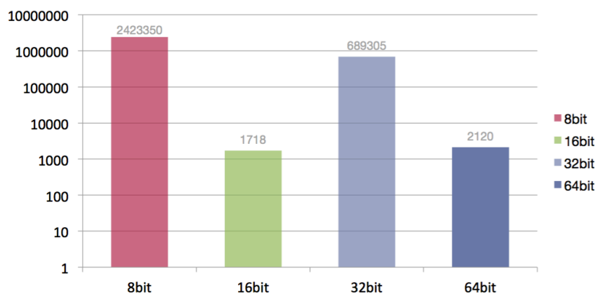
Figure 6-4. Memory access sizes (logarithmic scale).
