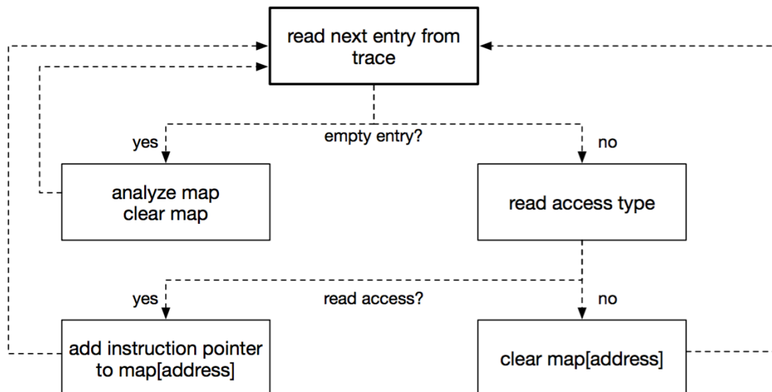
Figure 5-4. Conservative double fetch analysis. Interweaved reads and writes and overlapping memory accesses are ignored.
