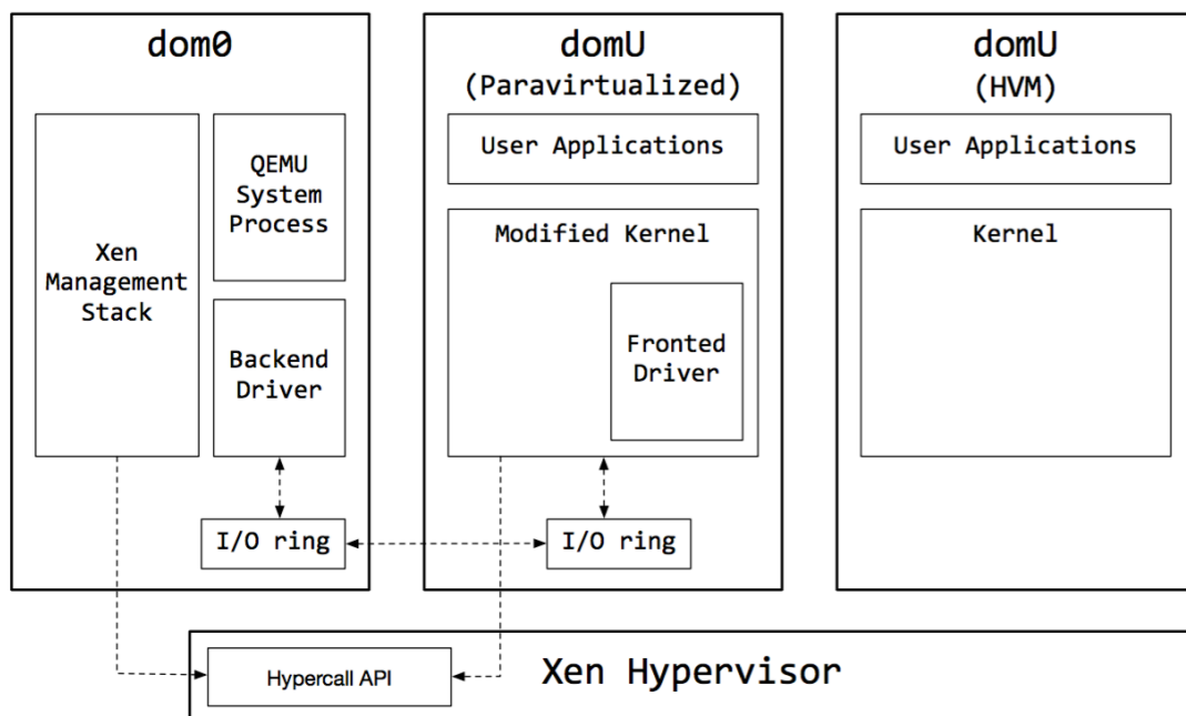
Figure 2-4. Xen architecture
