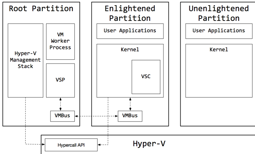
Figure 2-5. Hyper-V architecture
