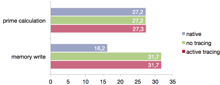
Figure 6-1. Sysbench CPU and memory benchmarks. Average runtime in seconds.
