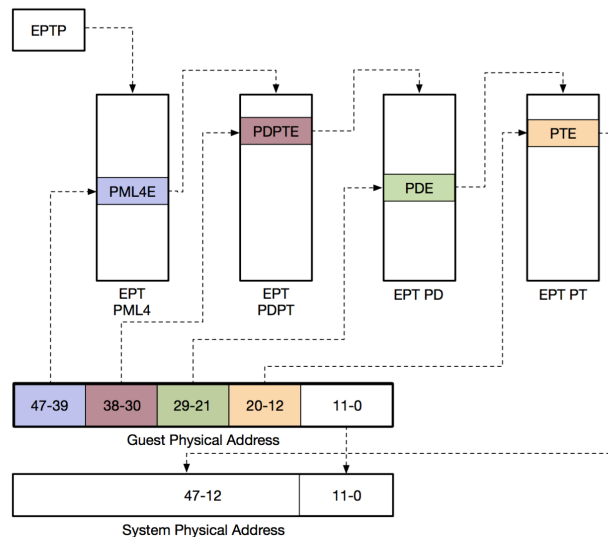
Figure 2-2. Intel EPT Address Translation.
