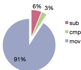
Figure 6-5. Ratio of instruction opcodes accessing shared memory.
