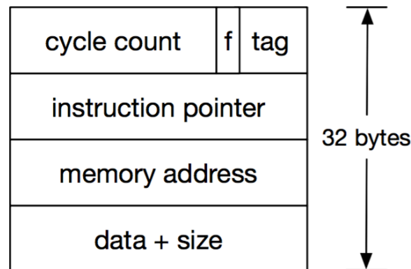
Figure 5-2. Layout of a memory trace entry.
