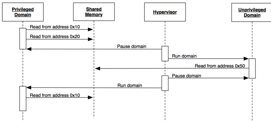
Figure 4-2. Double fetch: False negative.
