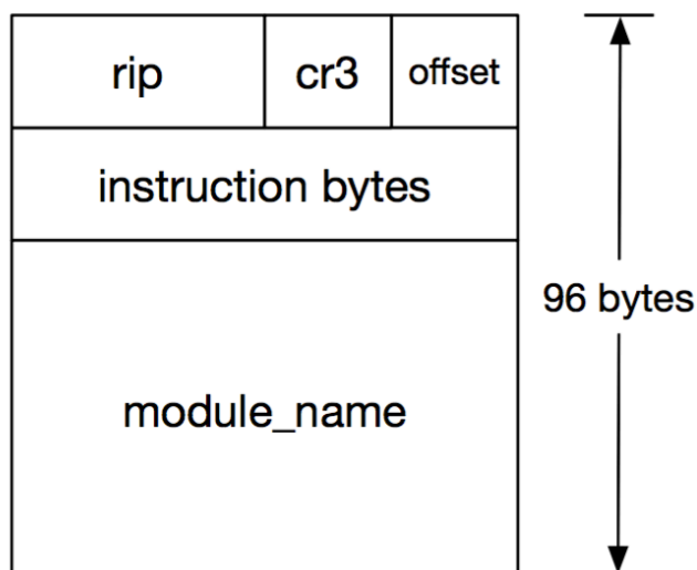
Figure 5-3. Layout of an instruction trace entry.
