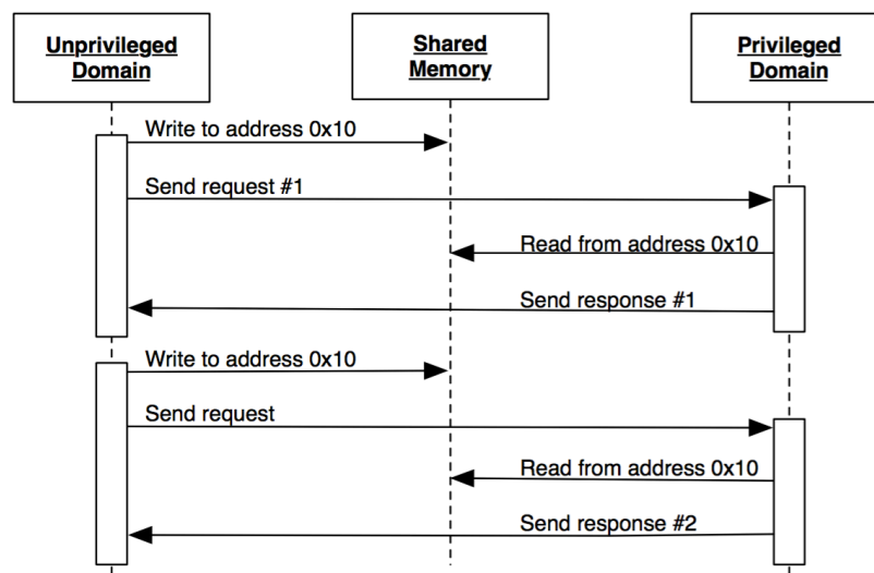
Figure 4-1. Double fetch: False positive.
